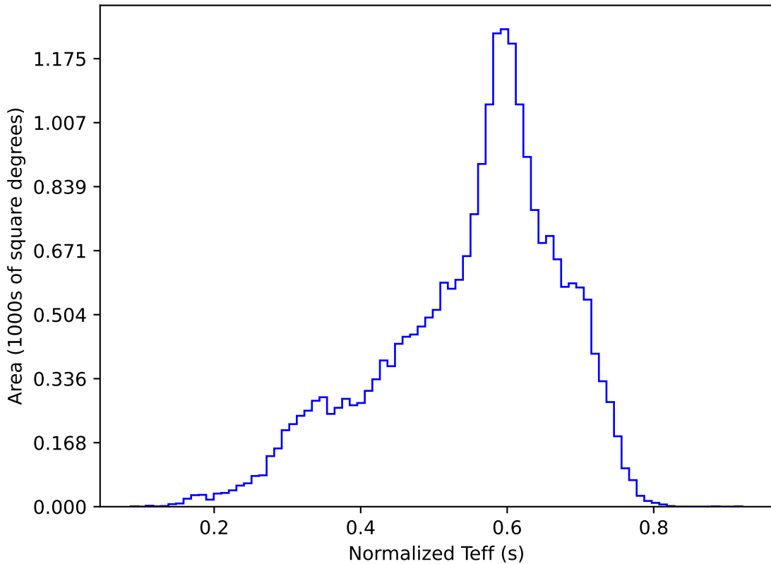
noroll_v3.4_10yrs All sky y band: Normalized Teff
