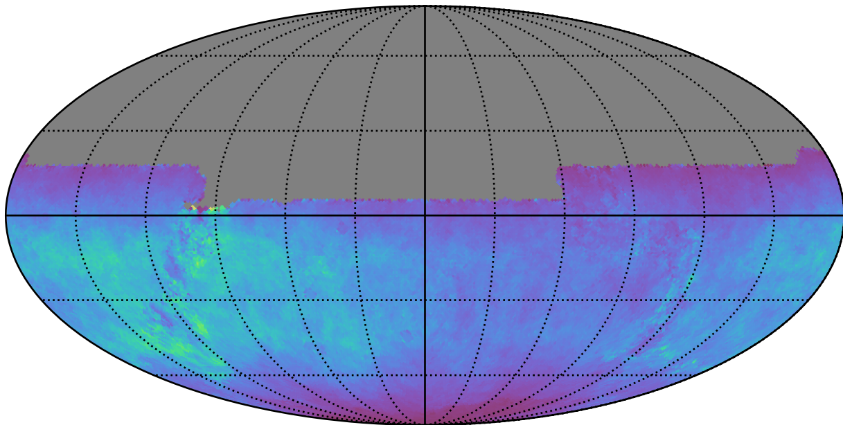
noroll_v3.4_10yrs All sky u band: Normalized Teff
