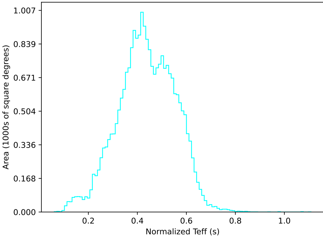
noroll_v3.4_10yrs All sky u band: Normalized Teff
