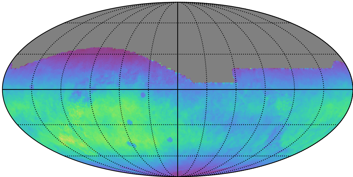
noroll_v3.4_10yrs All sky r band: Normalized Teff
