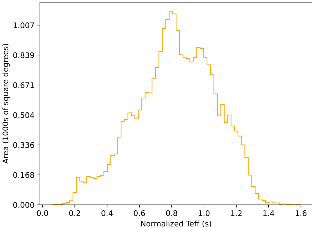
noroll_v3.4_10yrs All sky r band: Normalized Teff
