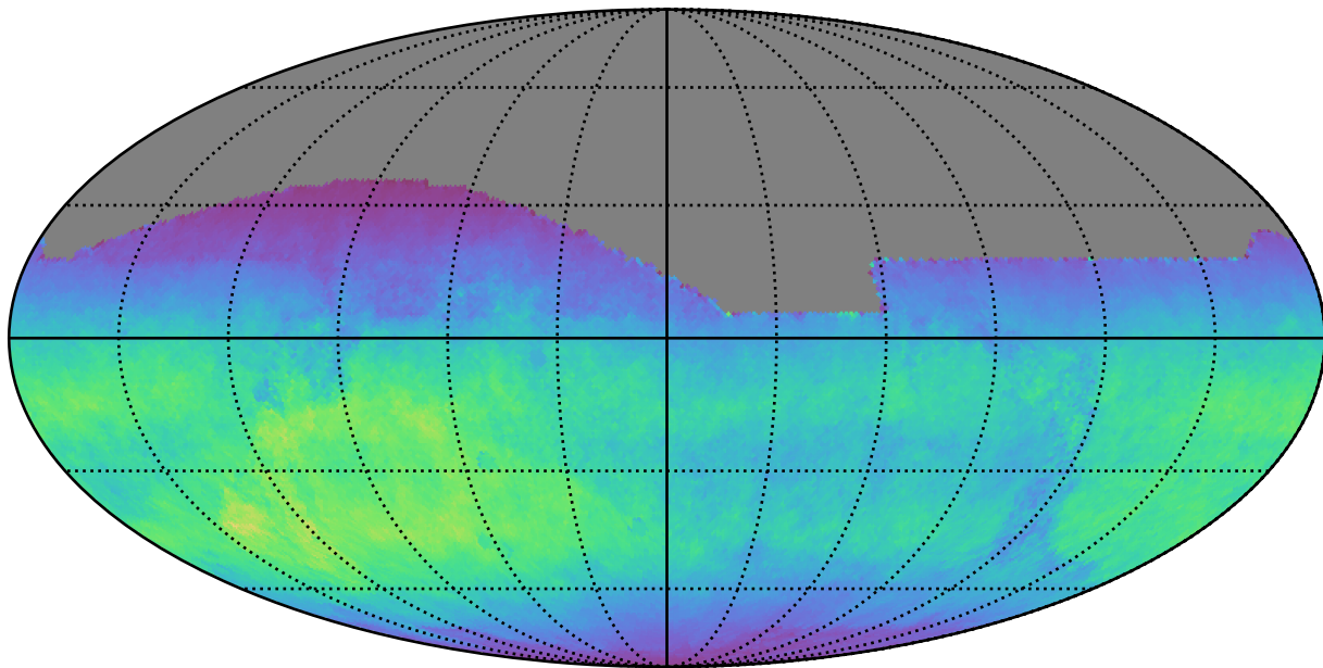
noroll_v3.4_10yrs All sky i band: Normalized Teff
