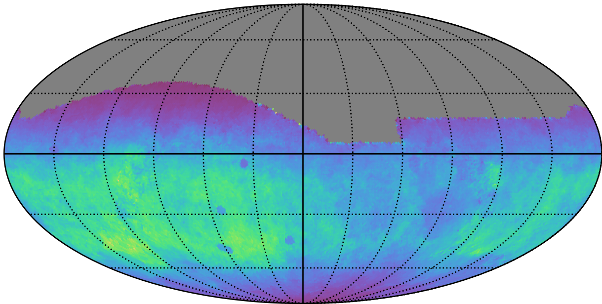
noroll_v3.4_10yrs All sky g band: Normalized Teff
