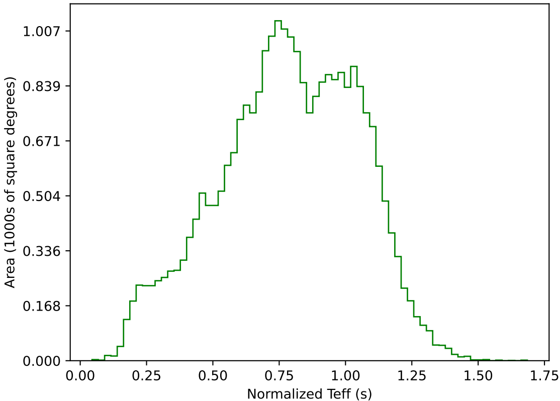
noroll_v3.4_10yrs All sky g band: Normalized Teff
