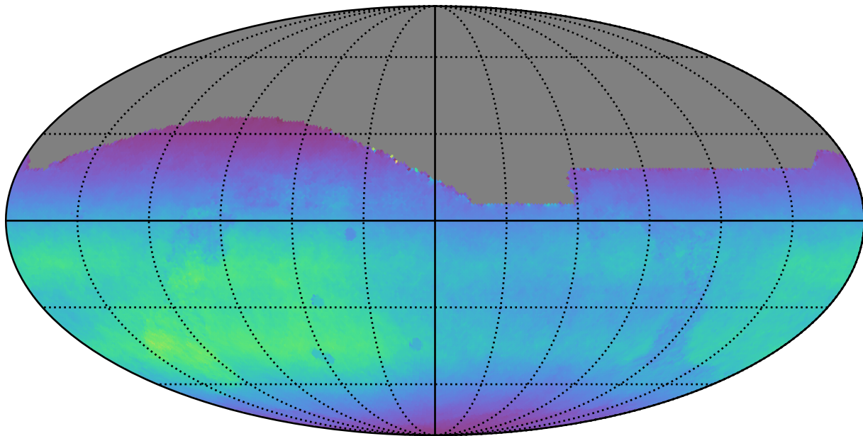
noroll_v3.4_10yrs All sky all bands: Normalized Teff
