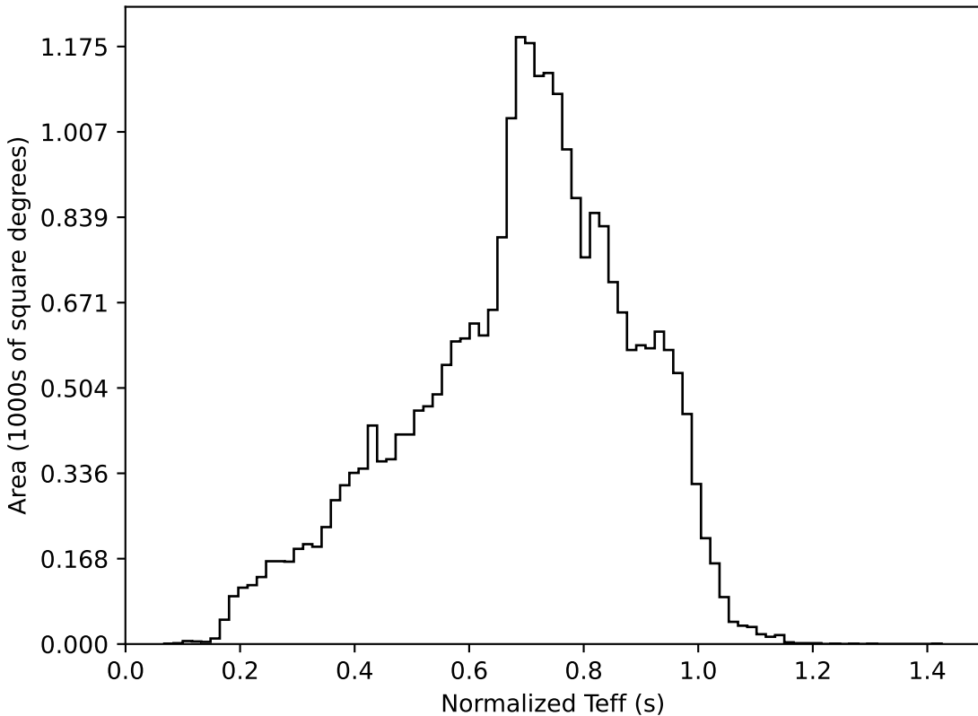
noroll_v3.4_10yrs All sky all bands: Normalized Teff
