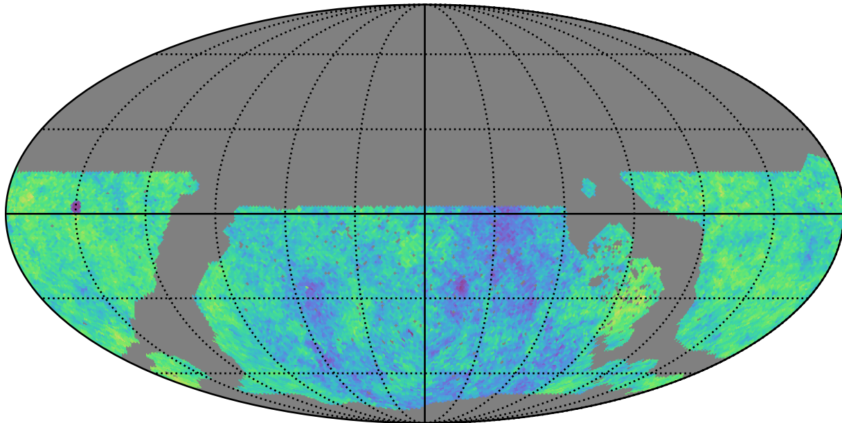
noroll_v3.4_10yrs WFD: Normalized Proper Motion Uncert @ 24.0
