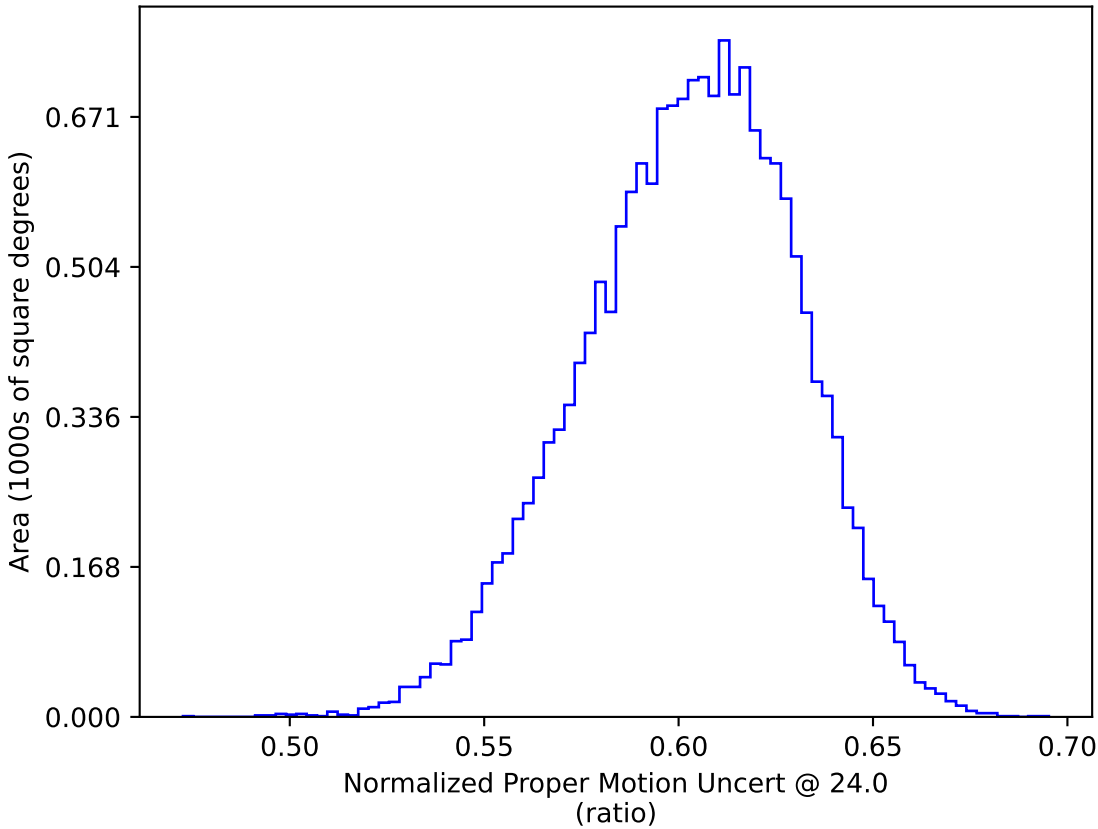
noroll_v3.4_10yrs WFD: Normalized Proper Motion Uncert @ 24.0
