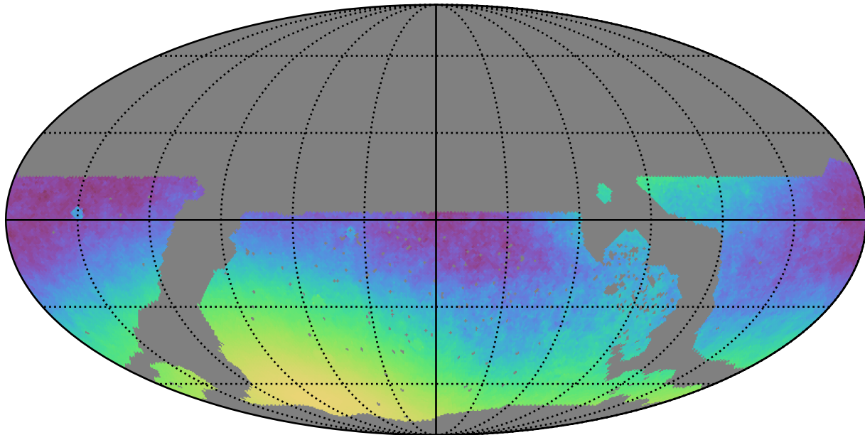
noroll_v3.4_10yrs WFD: Normalized Parallax Uncert @ 24.0
