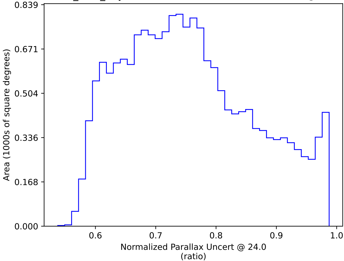
noroll_v3.4_10yrs WFD: Normalized Parallax Uncert @ 24.0
