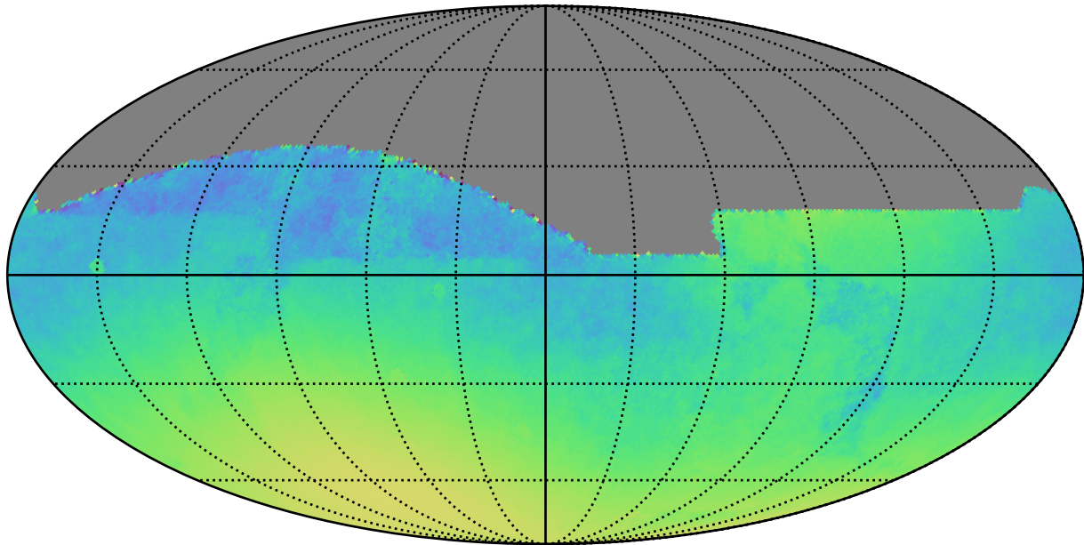
noroll_v3.4_10yrs All sky: Normalized Parallax Uncert @ 24.0
