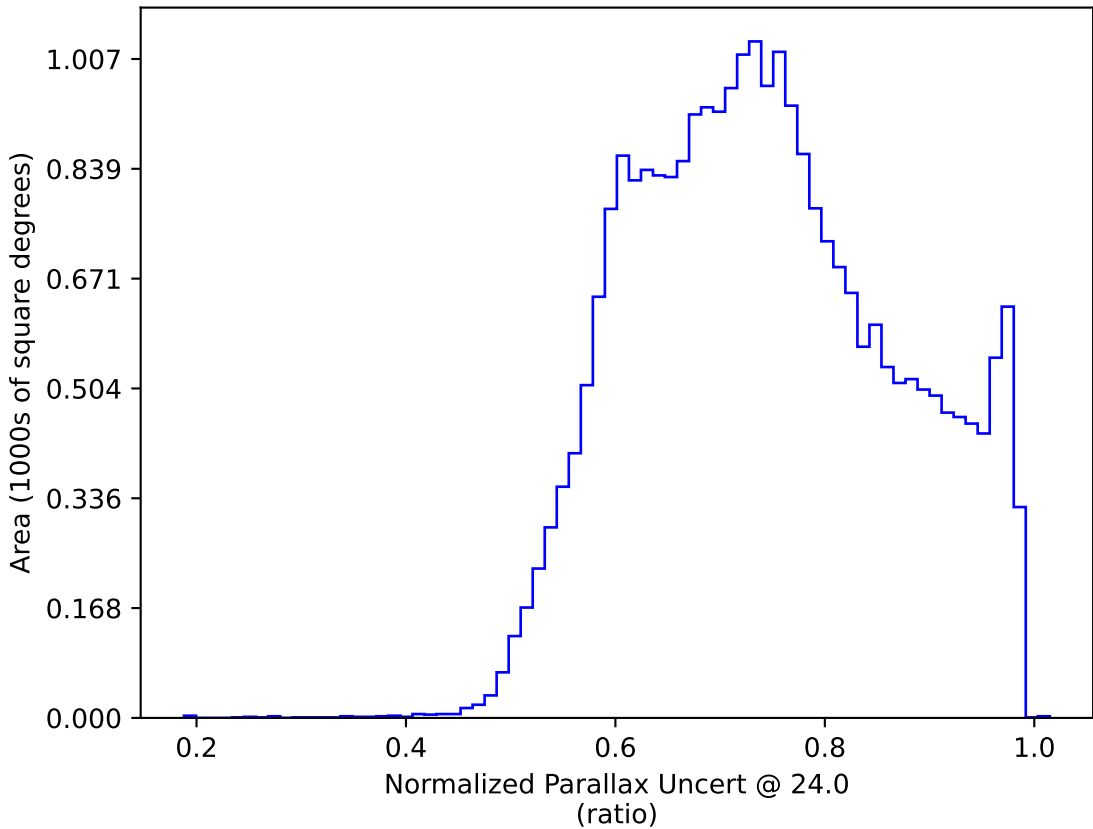
noroll_v3.4_10yrs All sky: Normalized Parallax Uncert @ 24.0
