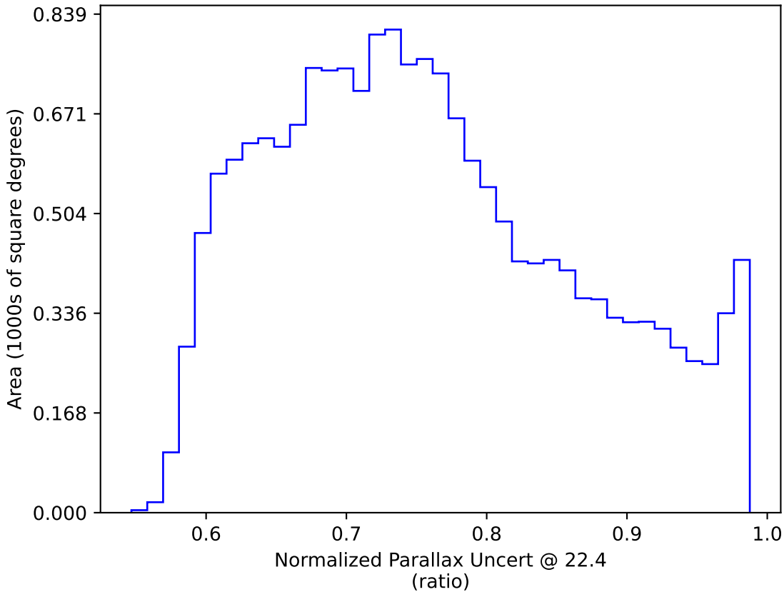
noroll_v3.4_10yrs WFD: Normalized Parallax Uncert @ 22.4
