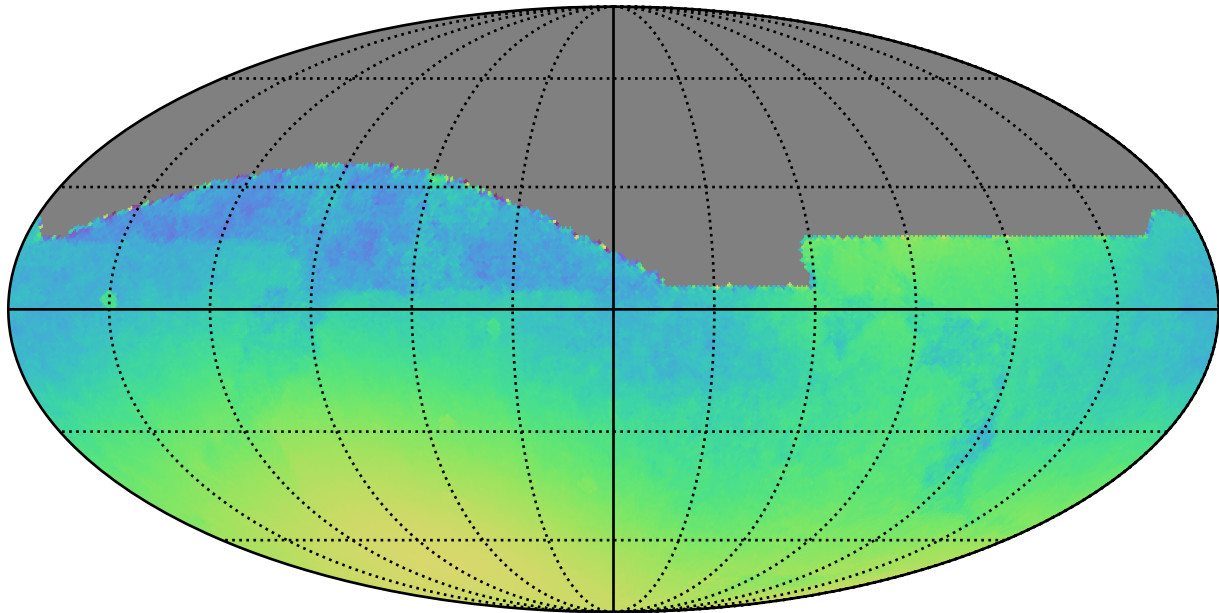
noroll_v3.4_10yrs All sky: Normalized Parallax Uncert @ 22.4
