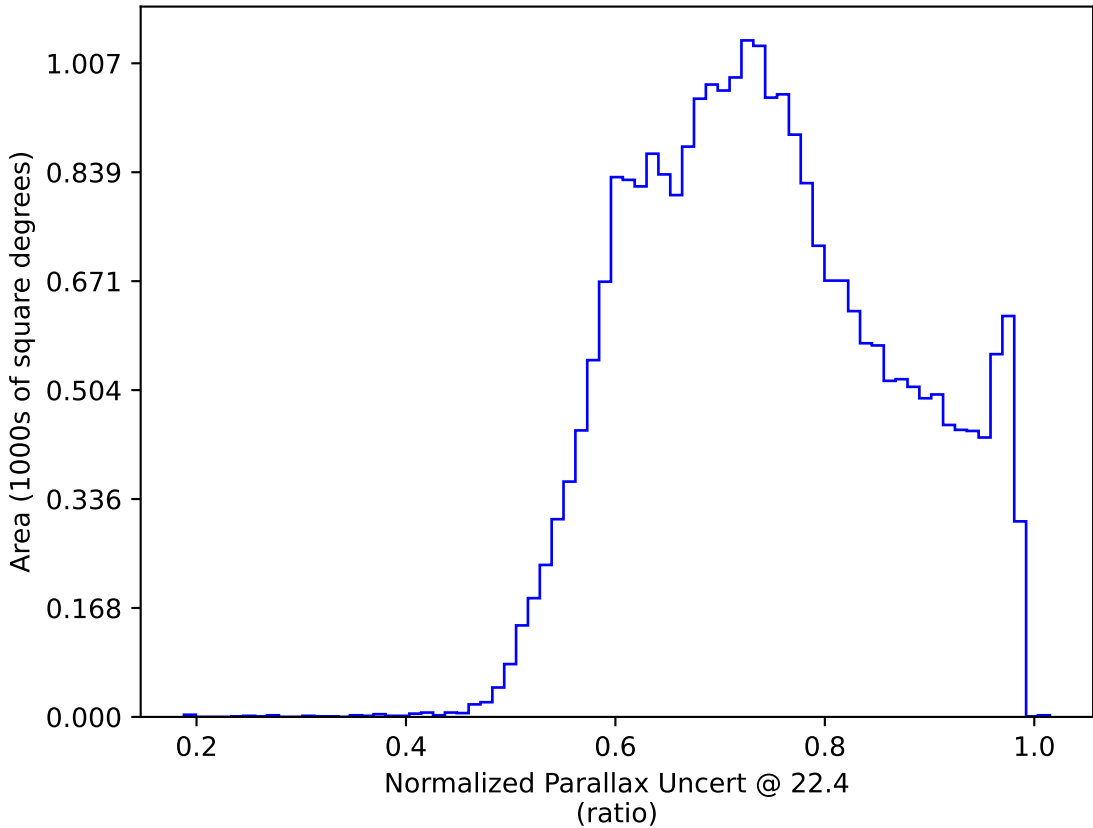
noroll_v3.4_10yrs All sky: Normalized Parallax Uncert @ 22.4
