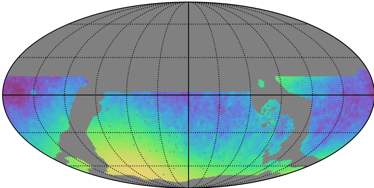
noroll_v3.4_10yrs WFD y band only: Normalized Parallax Uncert @ 21.3
