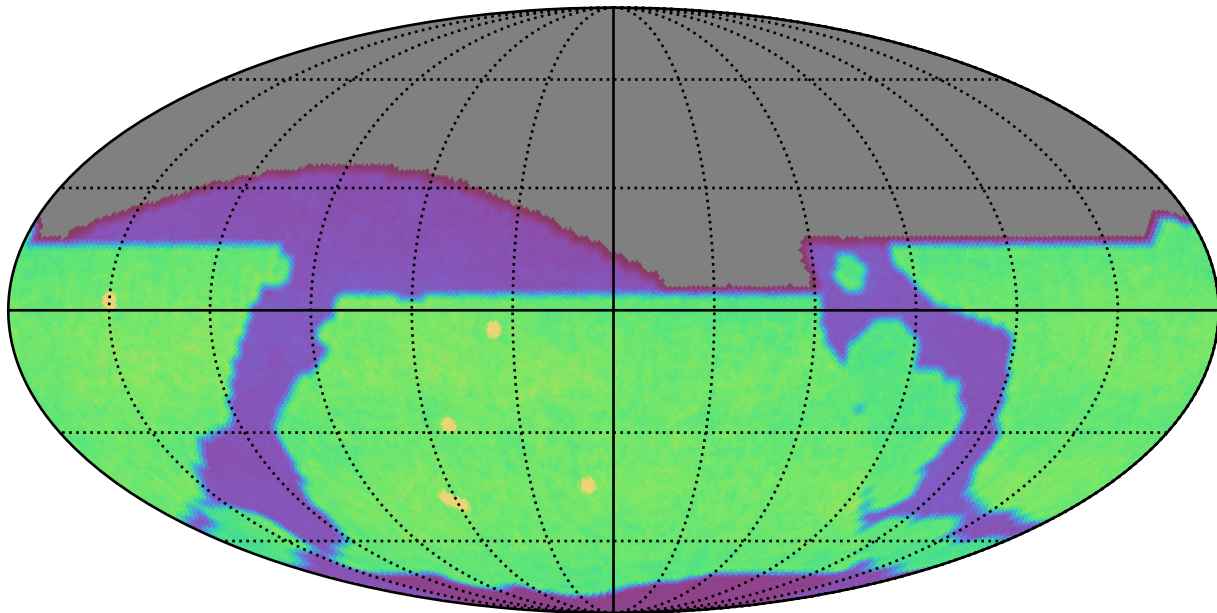
noroll_v3.4_10yrs All sky all bands: N Unique Nights
