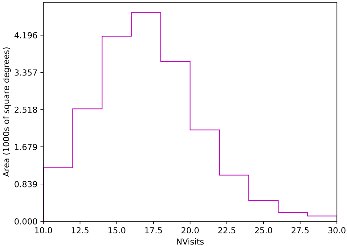
noroll_v3.4_10yrs Yr 3-4 z band: NVisits
