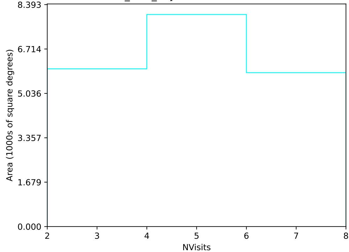
noroll_v3.4_10yrs Yr 3-4 u band: NVisits
