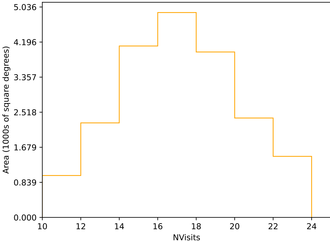
noroll_v3.4_10yrs Yr 3-4 r band: NVisits
