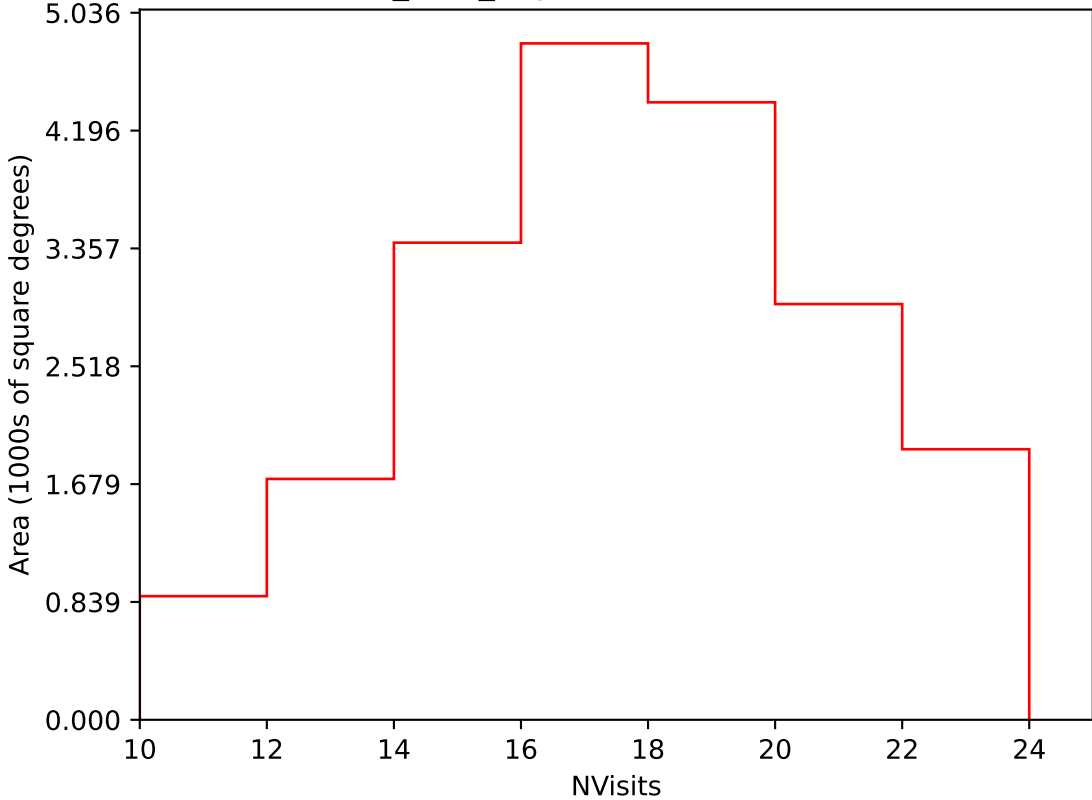
noroll_v3.4_10yrs Yr 3-4 i band: NVisits
