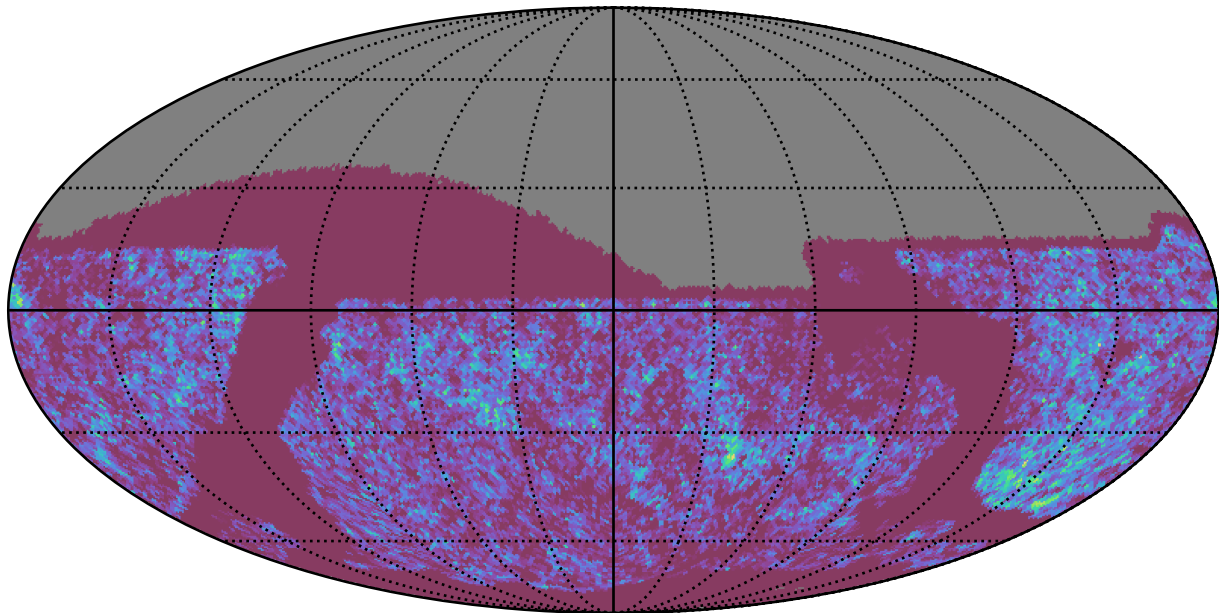
noroll_v3.4_10yrs Yr 3-4 all bands: NVisits
