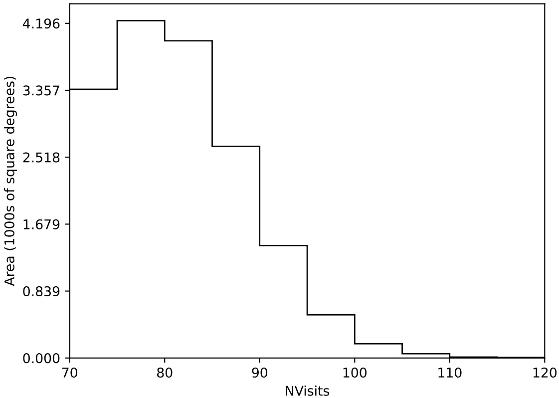
noroll_v3.4_10yrs Yr 3-4 all bands: NVisits
