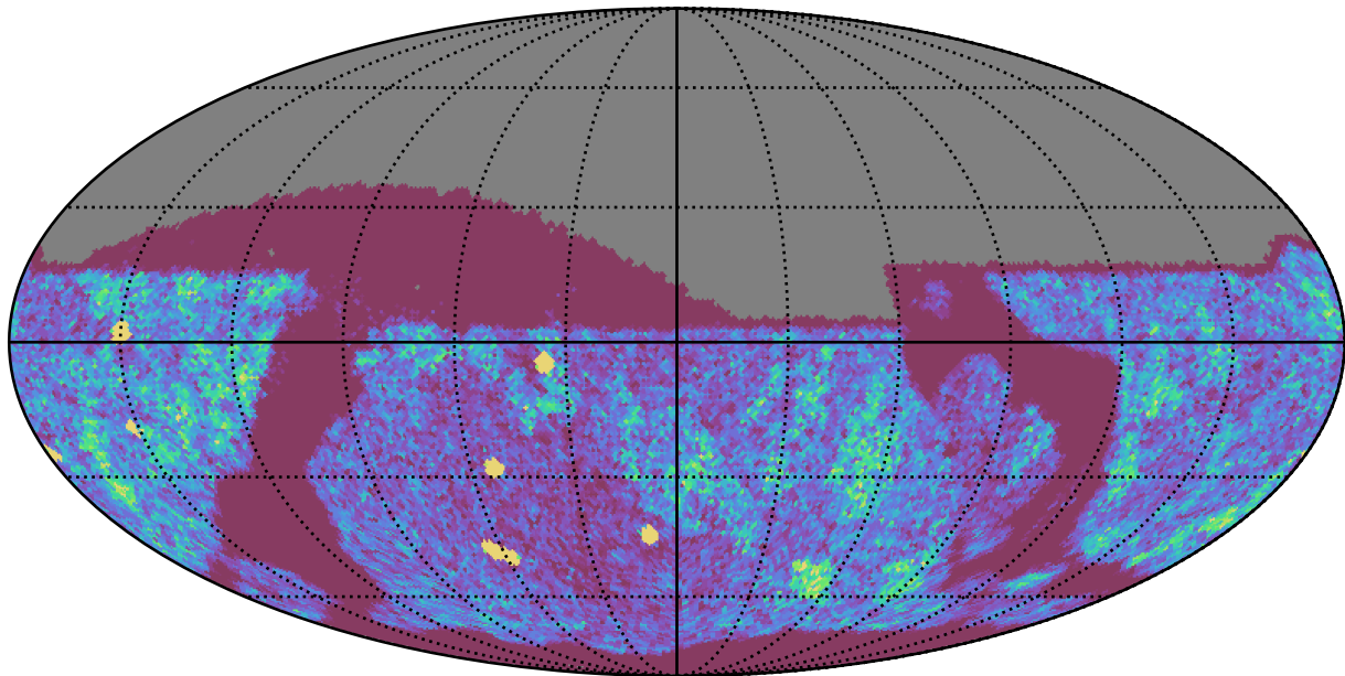
noroll_v3.4_10yrs Yr 1 z band: NVisits
