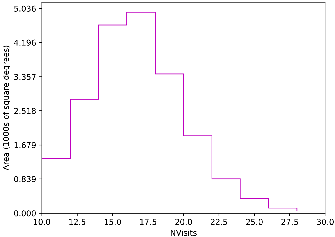
noroll_v3.4_10yrs Yr 1 z band: NVisits
