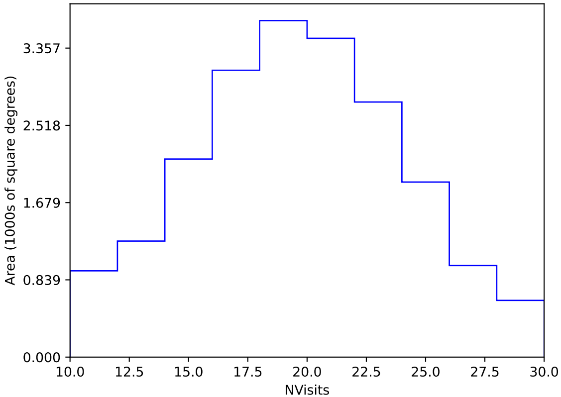
noroll_v3.4_10yrs Yr 1 y band: NVisits
