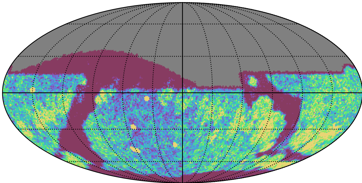
noroll_v3.4_10yrs Yr 1 r band: NVisits
