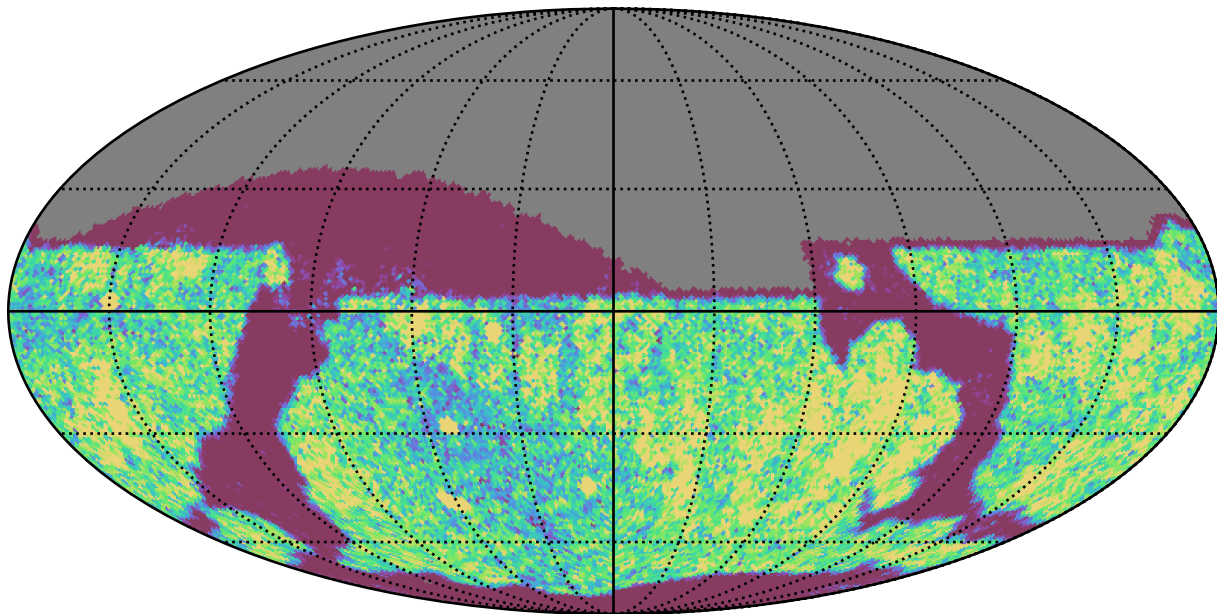
noroll_v3.4_10yrs Yr 1 i band: NVisits
