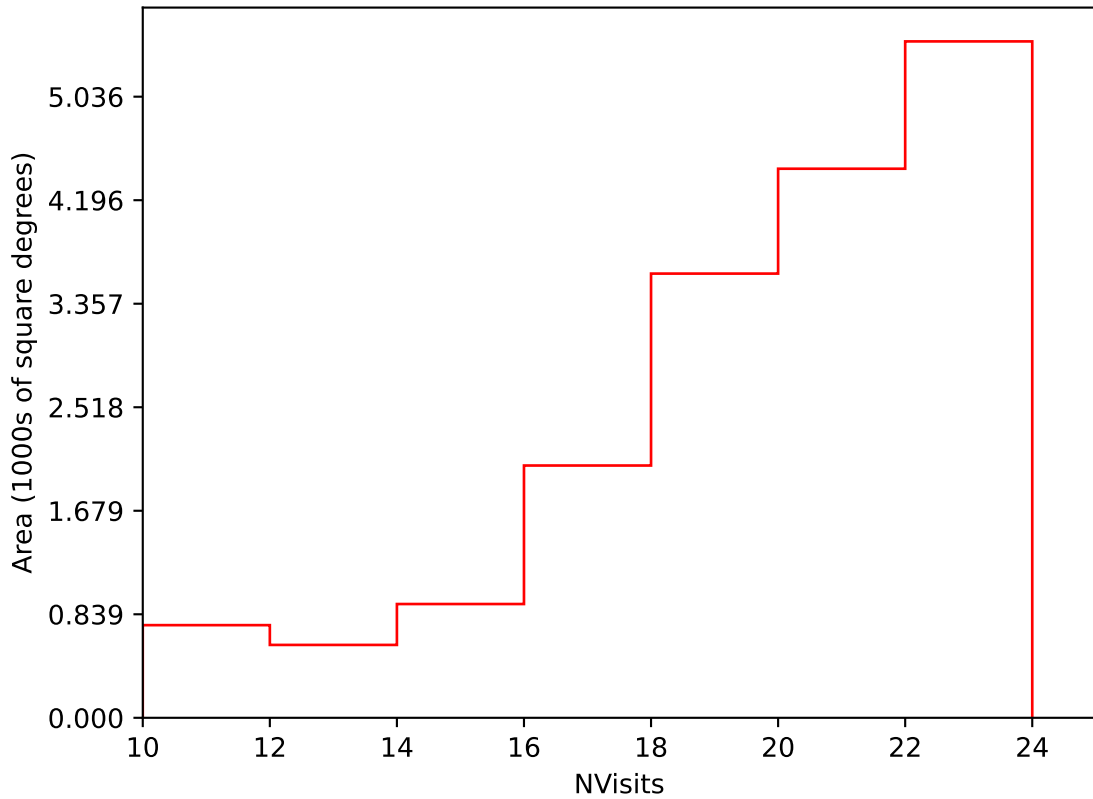
noroll_v3.4_10yrs Yr 1 i band: NVisits
