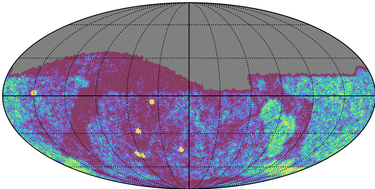
noroll_v3.4_10yrs Yr 1 g band: NVisits
