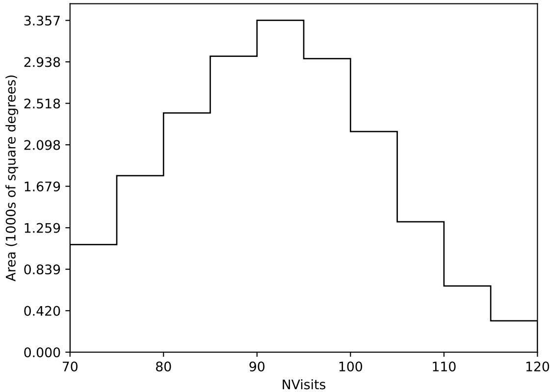
noroll_v3.4_10yrs Yr 1 all bands: NVisits
