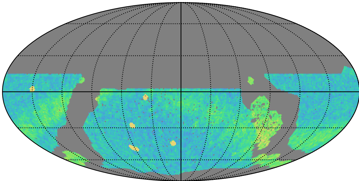
noroll_v3.4_10yrs WFD r band: NVisits
