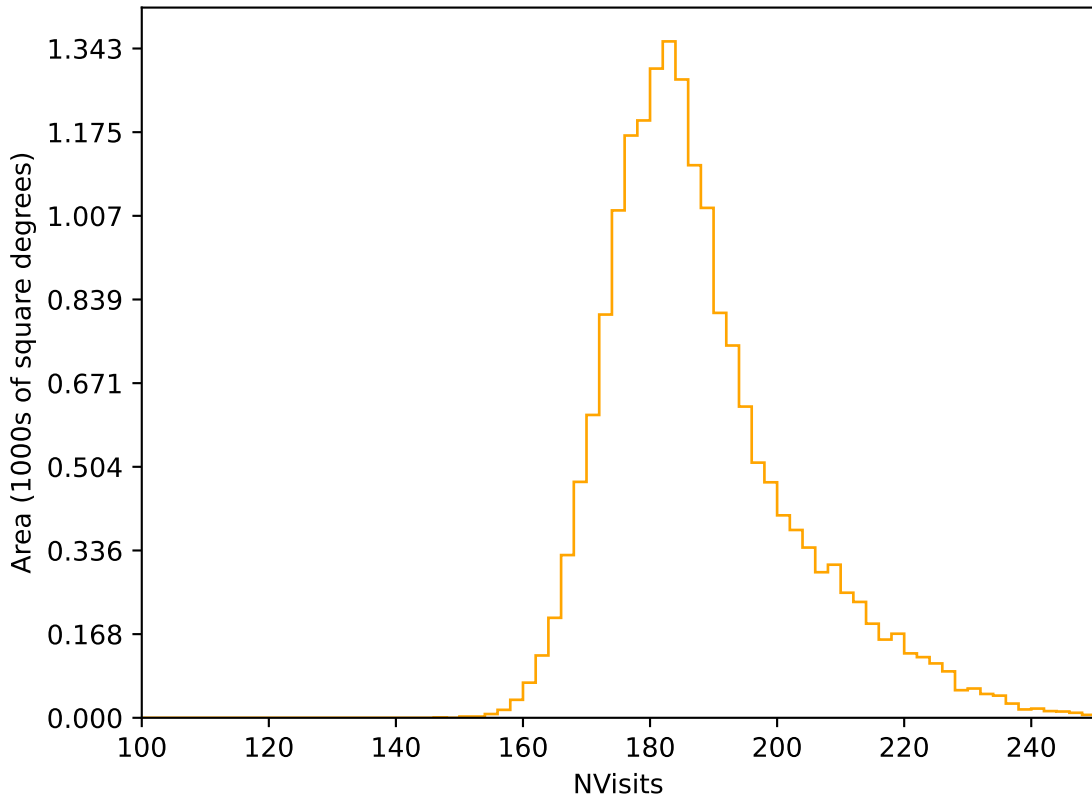
noroll_v3.4_10yrs WFD r band: NVisits
