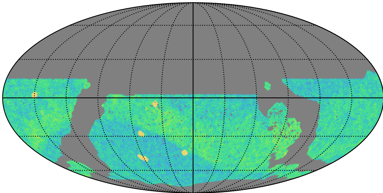
noroll_v3.4_10yrs WFD i band: NVisits
