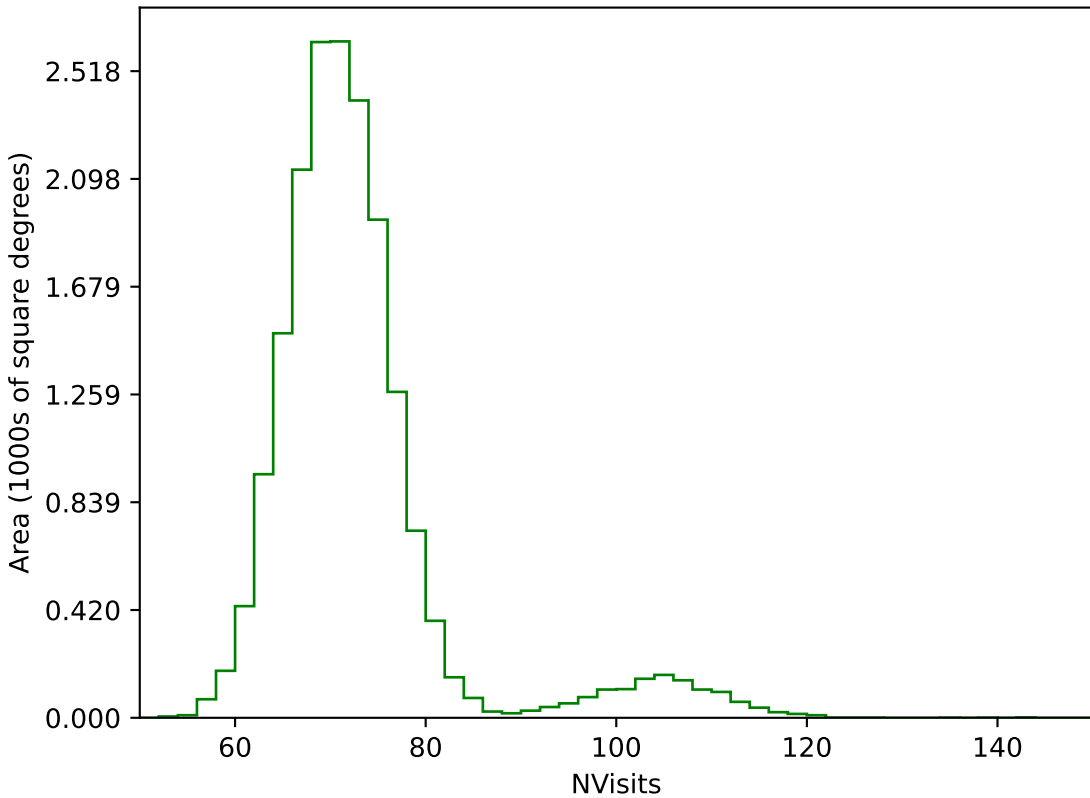
noroll_v3.4_10yrs WFD g band: NVisits
