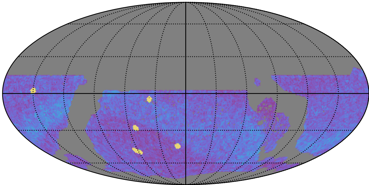
noroll_v3.4_10yrs WFD all bands: NVisits
