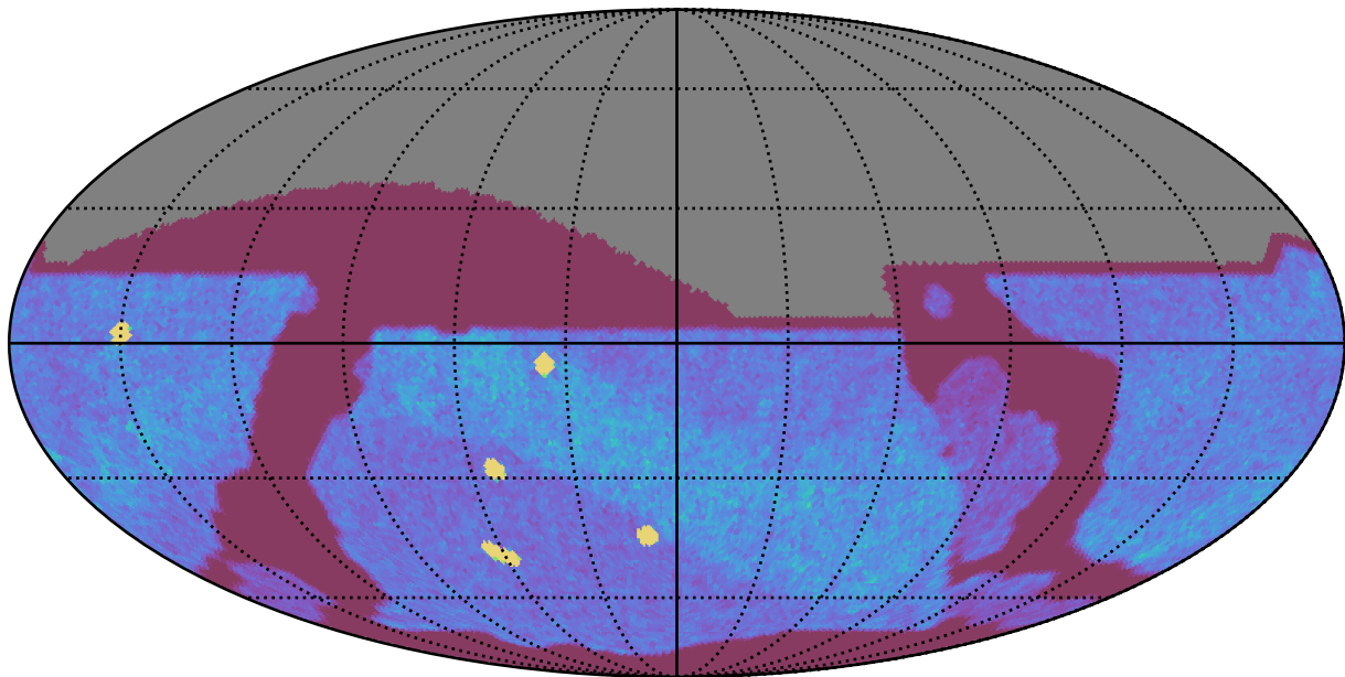
noroll_v3.4_10yrs All sky z band: NVisits
