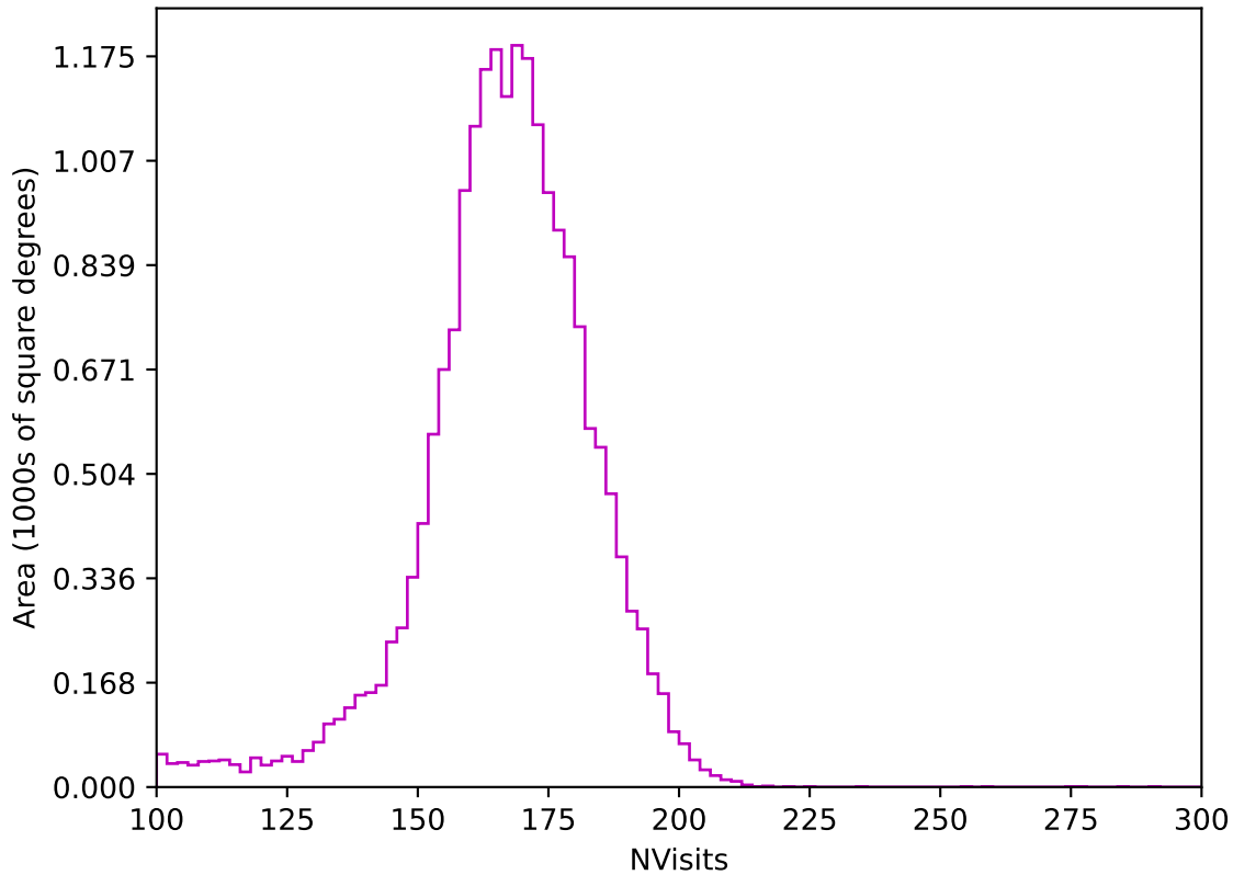
noroll_v3.4_10yrs All sky z band: NVisits
