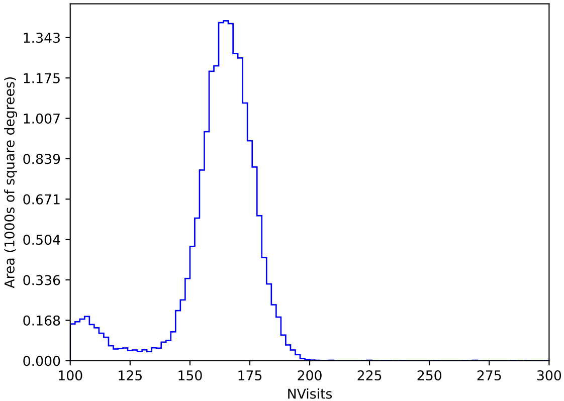
noroll_v3.4_10yrs All sky y band: NVisits
