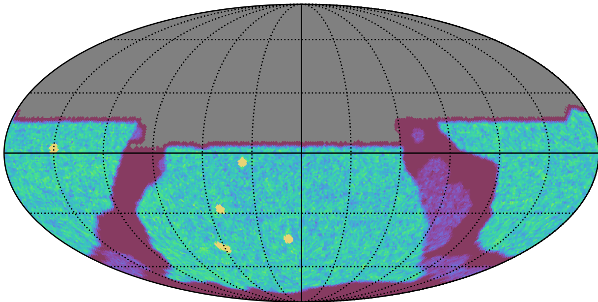
noroll_v3.4_10yrs All sky u band: NVisits
