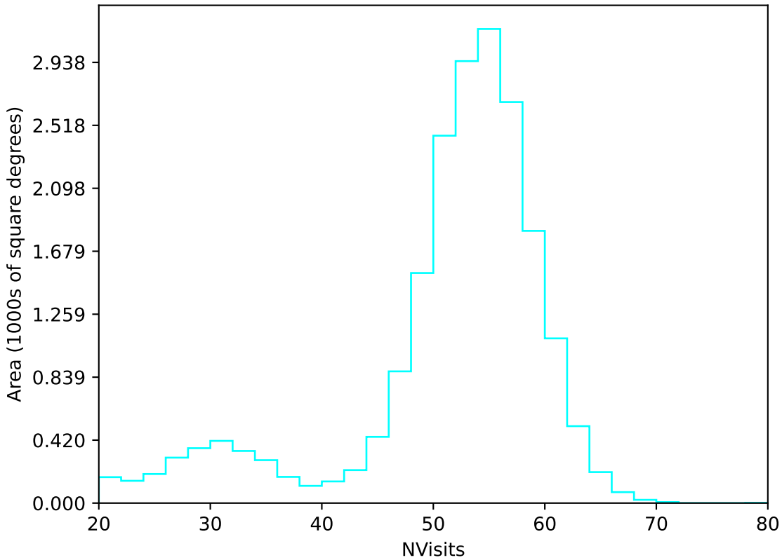
noroll_v3.4_10yrs All sky u band: NVisits
