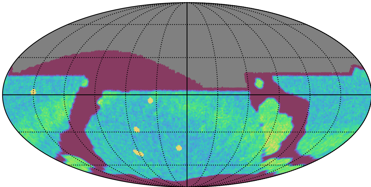
noroll_v3.4_10yrs All sky r band: NVisits
