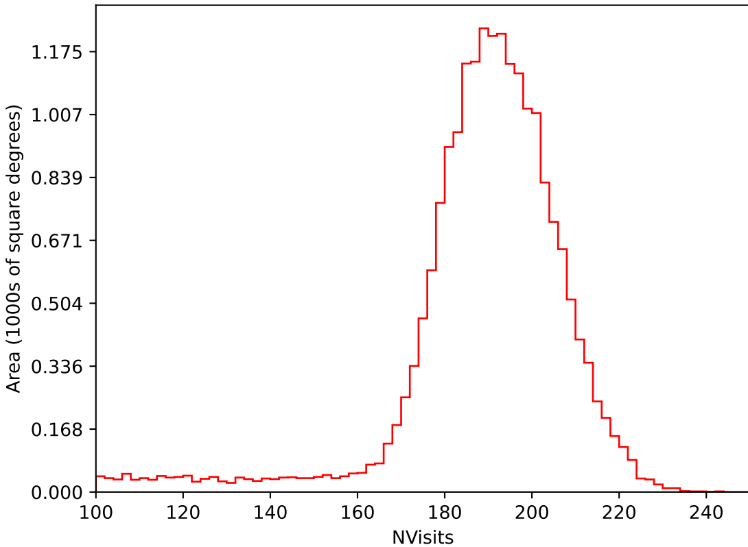
noroll_v3.4_10yrs All sky i band: NVisits
