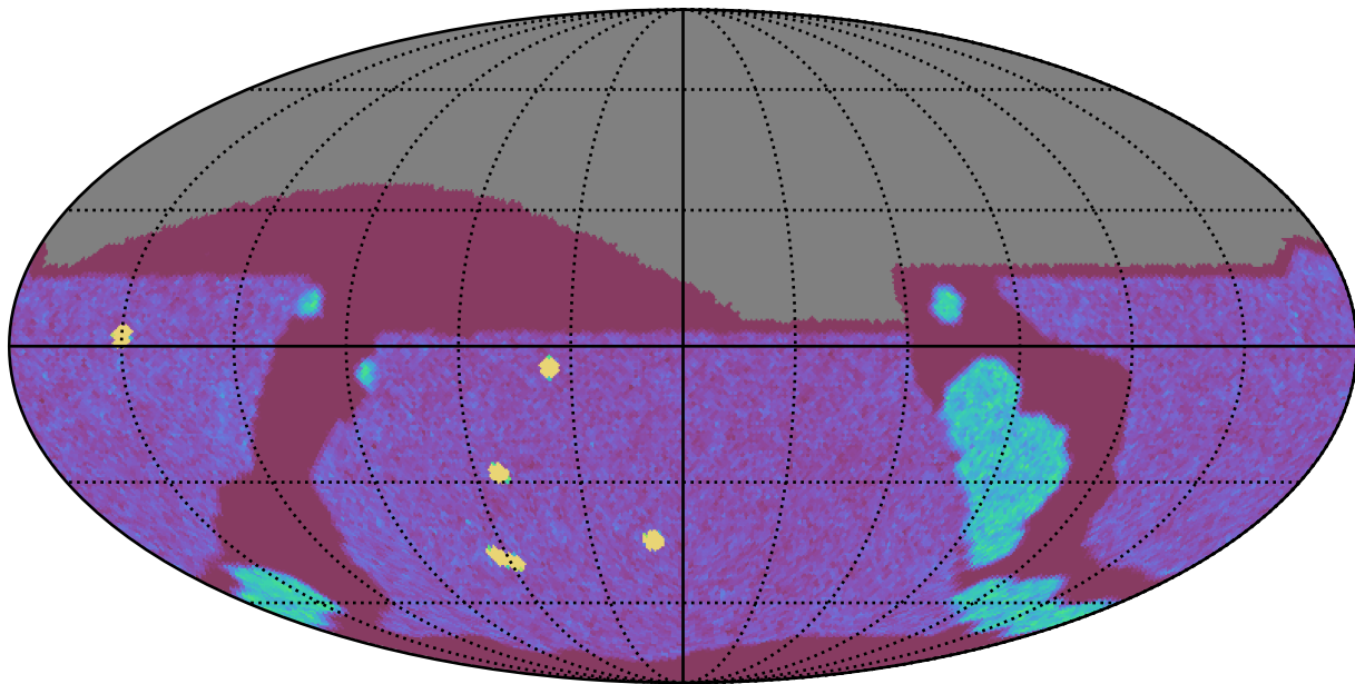
noroll_v3.4_10yrs All sky g band: NVisits
