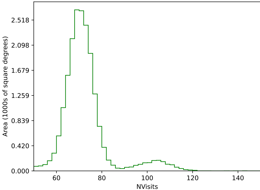
noroll_v3.4_10yrs All sky g band: NVisits
