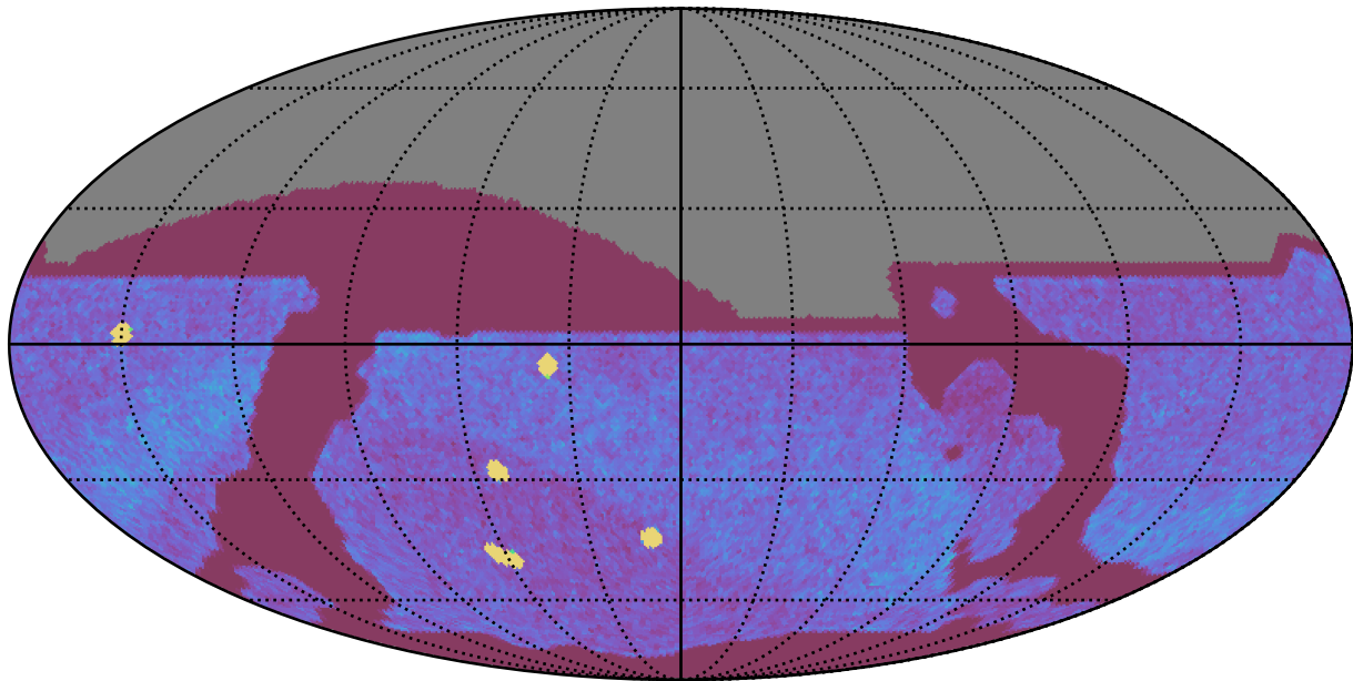
noroll_v3.4_10yrs All sky all bands: NVisits
